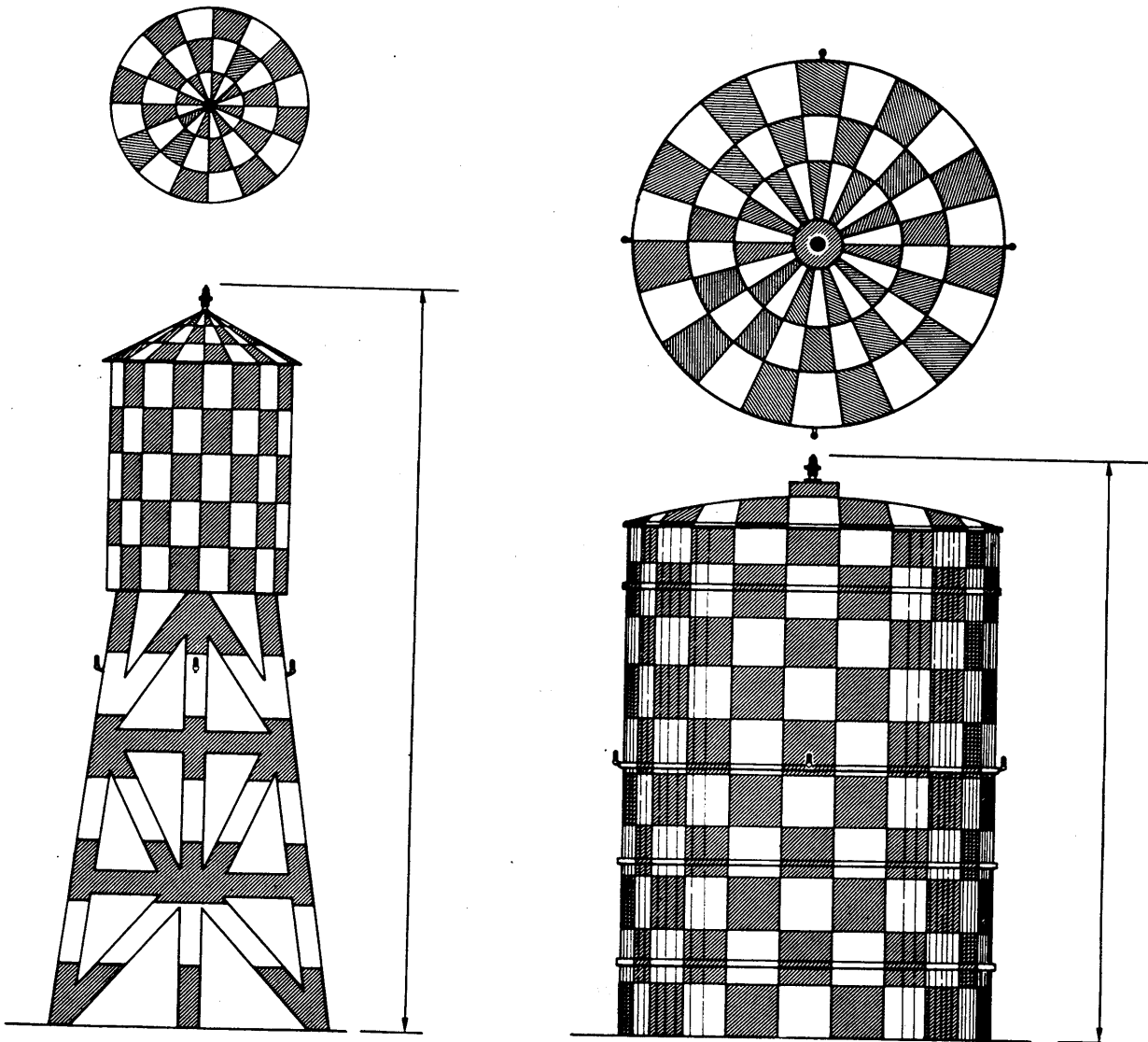
LIGHTING More than 150 ft. (45m) but not more than 300 ft. (90m)
